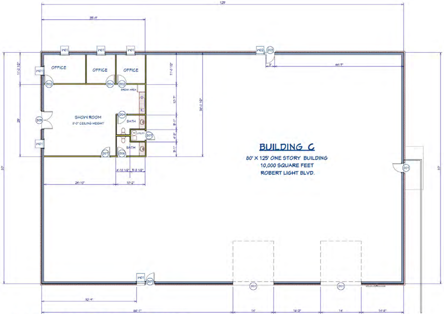
BUILDING-C FLOOR PLAN
